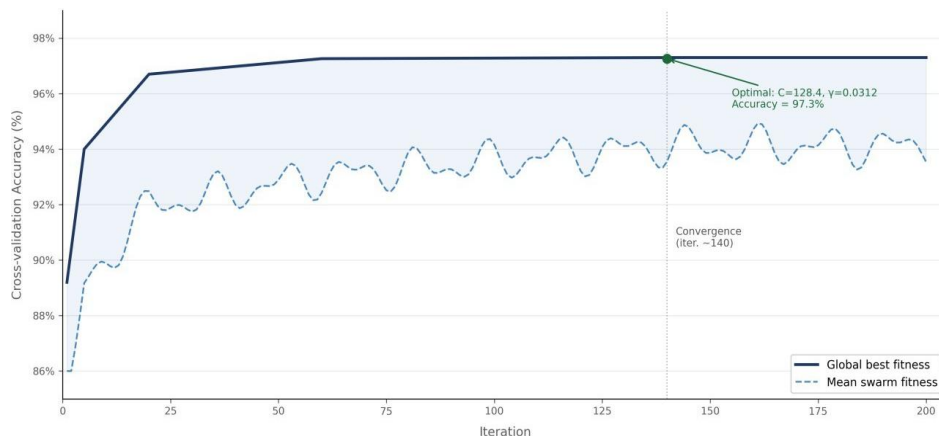
Fig. 3. PSO convergence curve—best and mean swarm fitness over 200 iterations (Swarm size: 30 particles, inertia weight w : 0.9–0.4, c_1 = c_2 = 2.0 ).
