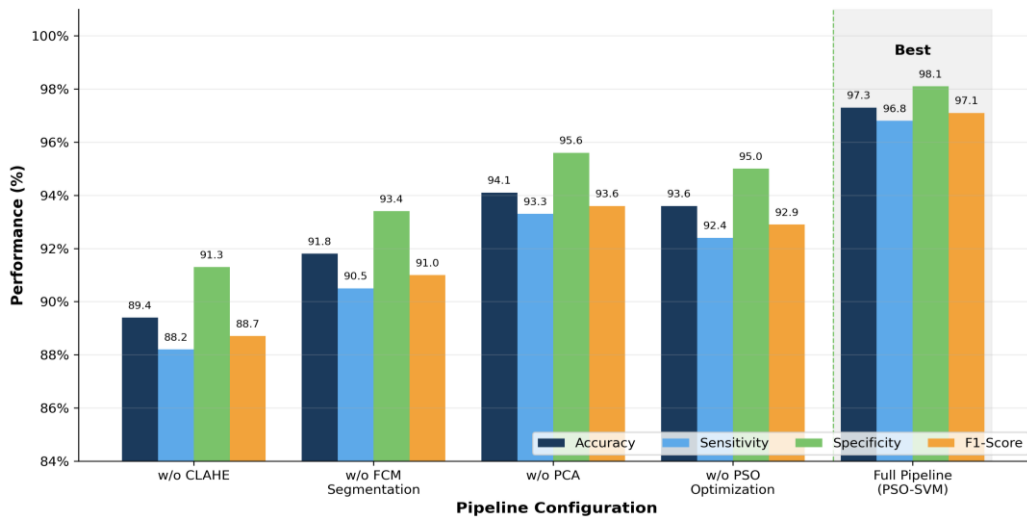
Fig. 6. Ablation study—individual component contribution to PSO-SVM performance (each configuration removes one component while all others remain active).
