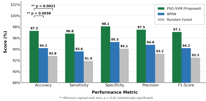
Fig. 5. Performance comparison of PSO-SVM vs. baseline classifiers (brackets indicate statistically significant difference, Wilcoxon signed-rank test).
