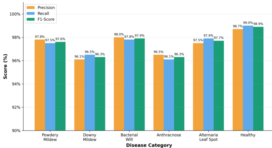
Fig. 7. Disease-wise precision, recall, and F1-Score of the PSO-SVM classifiers across different cucumber leaf conditions.
